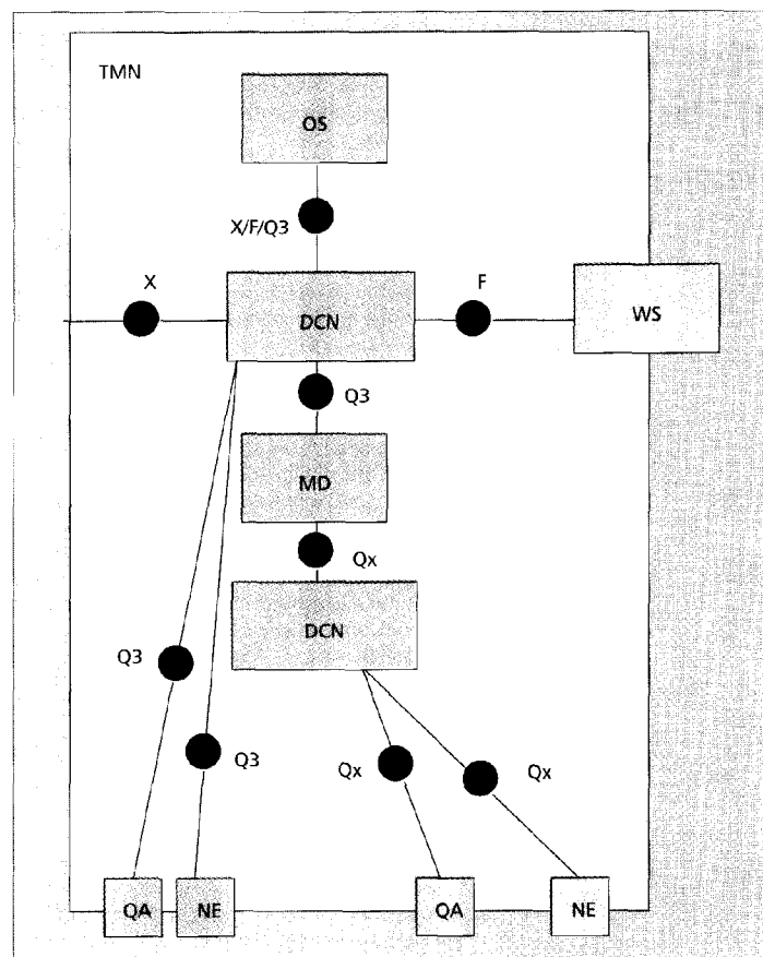
■ Figure 1. A simplified TMN physical architecture.
